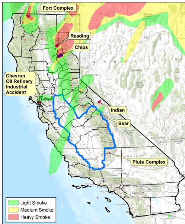
Figure 8b: Smoke plume impacting the San Joaquin Valley from the Chips and Bear Fires on August 8, 2012.
