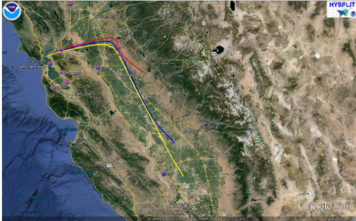
Figure 4: Forward Trajectories from the Richmond oil refinery industrial accident at 75 (red), 100 (blue), and 125 (yellow) meters on August 06, 2012.
