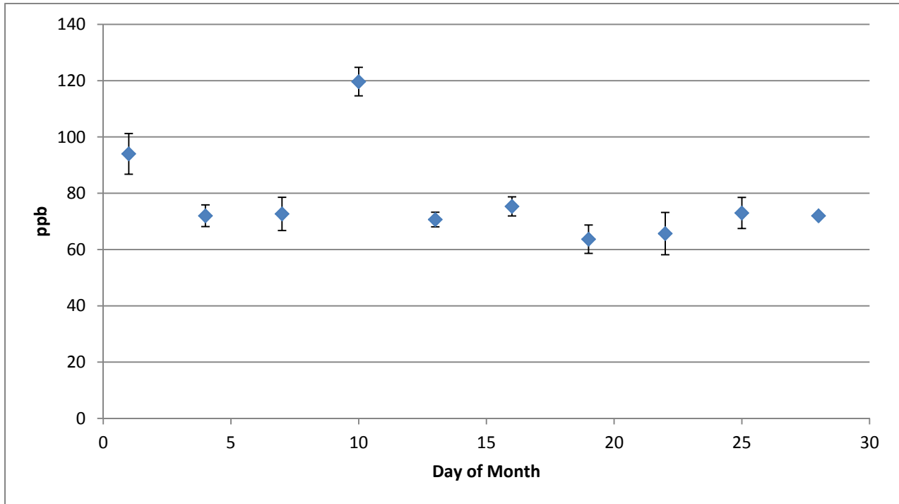
Figure 22: Fresno-Drummond, August 2012, 12:00 PM Measured Ozone Values, 3-Day Averages.
